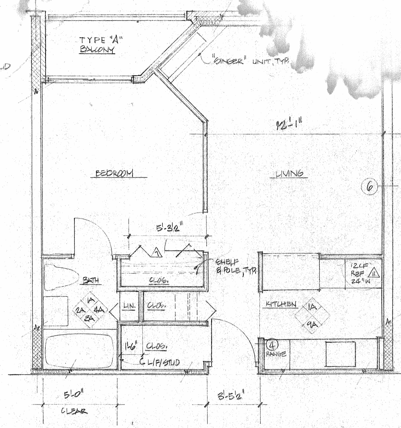
TYPE "H" DIMENSIONS SIM. TO "G" U.O.N.
