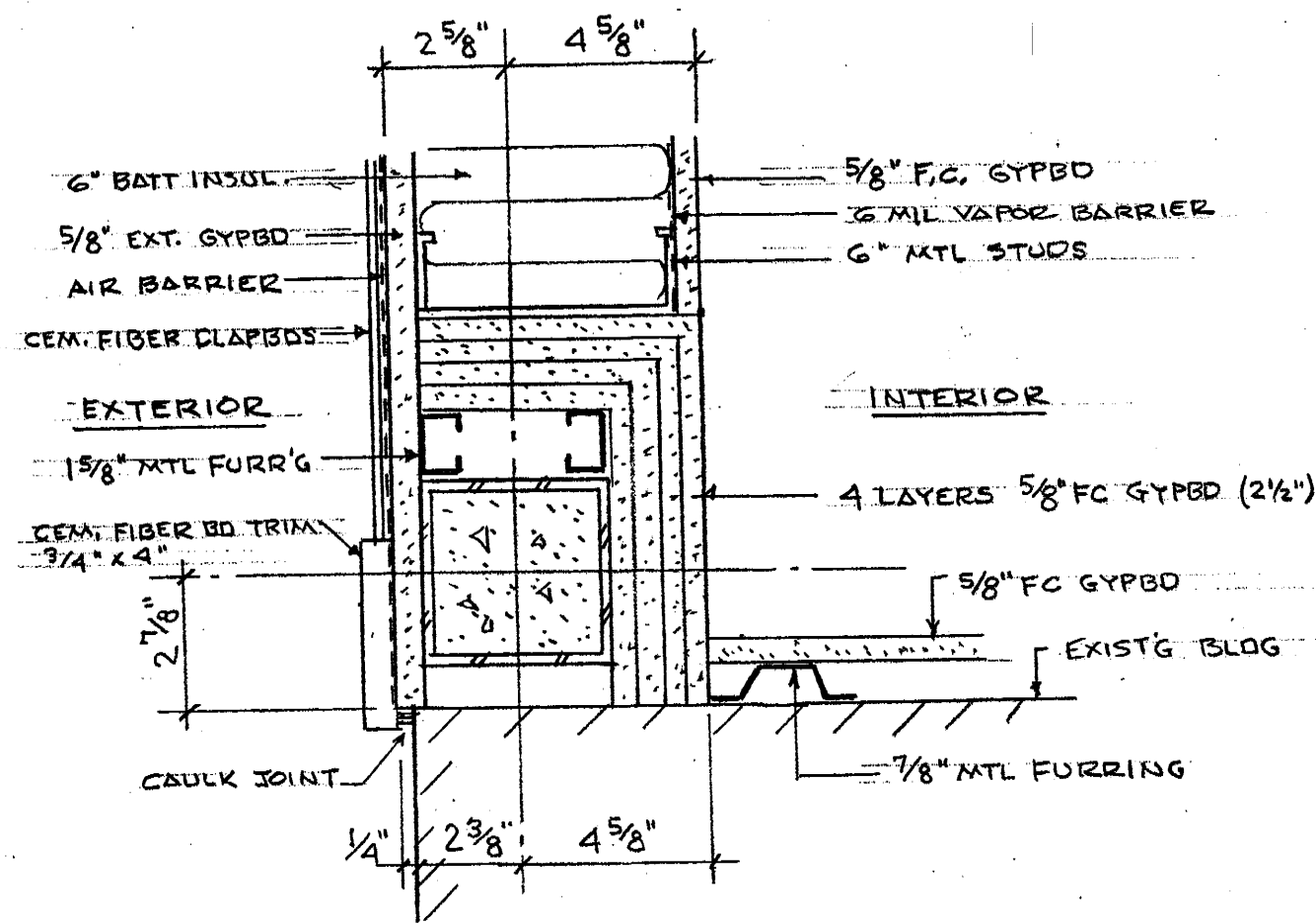
4 EXTERIOR WALL LALLY COLUMN FIREPROOF'G AT EXIST'G BLDG JUNCTION 3 HR RATED UL NO. X528 3"=1'-0"
