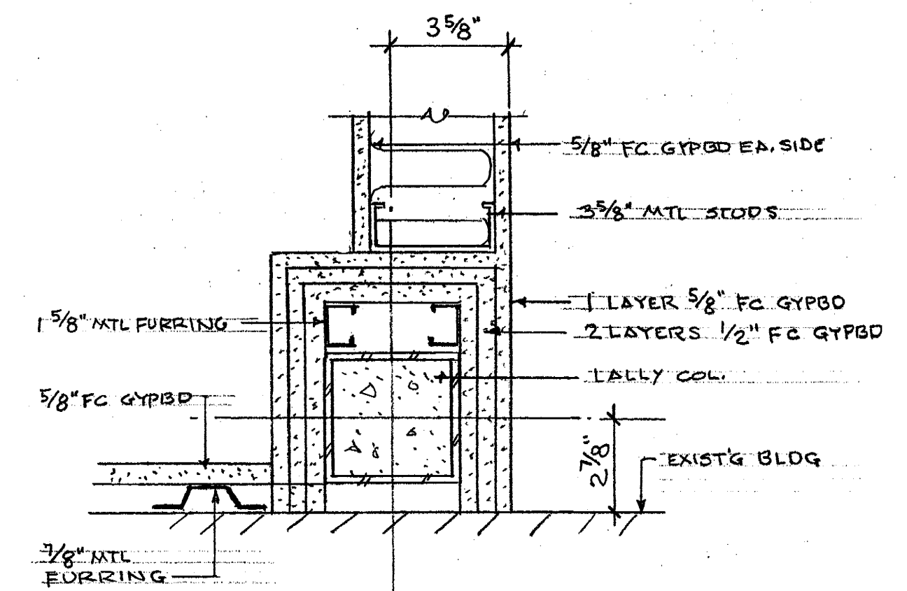
3 TYP. INTERIOR LALLY COL. FIREPROOF'G 2 HR RATED UL NO. X528 3"=1'-0"
