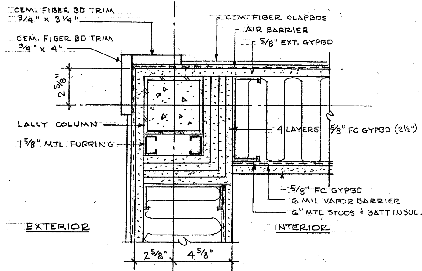
1 EXTERIOR CORNER WALL LALLY COLUMN FIREPROOF'G 3 HR RATED UL NO. X528 3"=1'-0"
