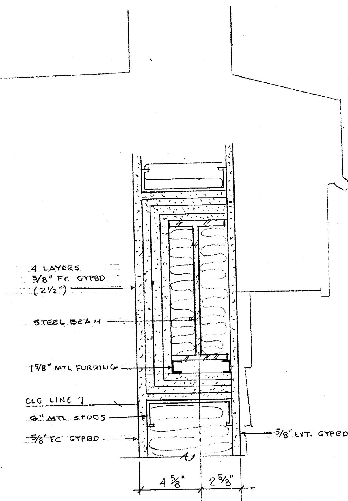
EXTERIOR WALL STEEL BEAM FIREPROOF'G 3 HR RATED UL NO. X528 3"=1'-0"
