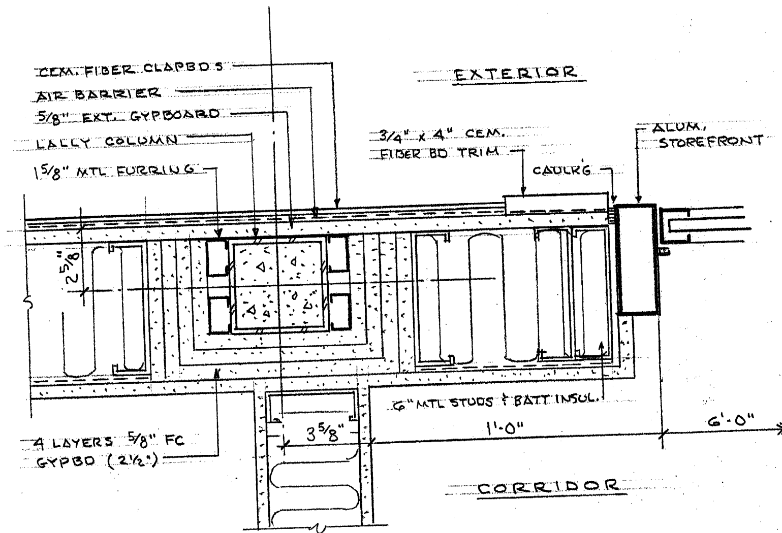
2 EXTERIOR WALL LALLY COL. FIREPROOF'G 3 HR RATED UL NO. X528 3"=1'-0"
