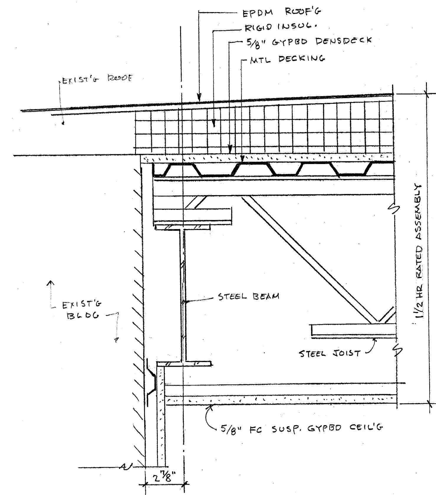
INTERIOR BEAM + JOIST FIRE RATED ASSEMBLY 1 1/2 HR ASSEMBLY UL NO. P510 3"=1'-0"
