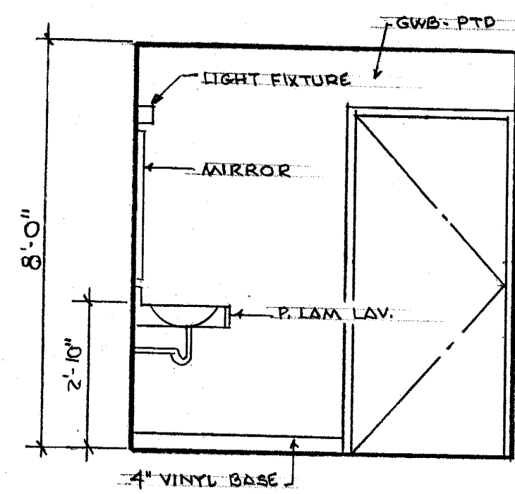
TYP. VISITOR HP TOILET AT CENTRAL CORE
