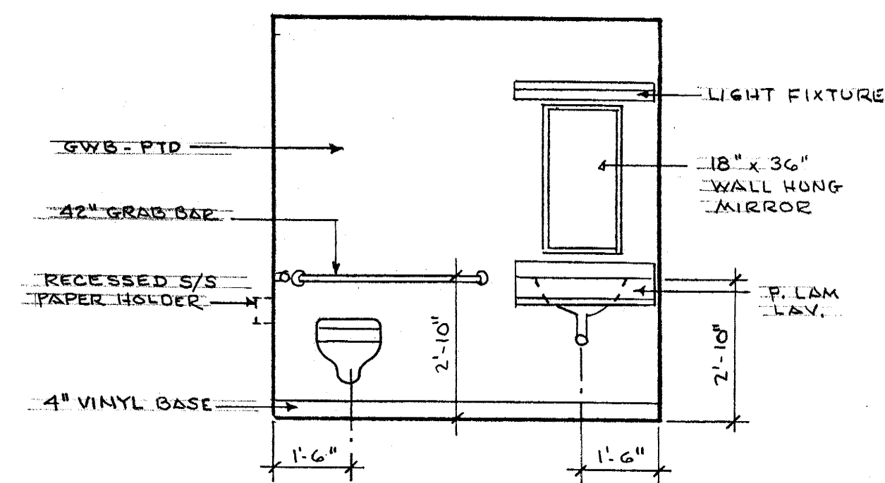
TYP. VISITOR HP TOILET AT CENTRAL CORE
