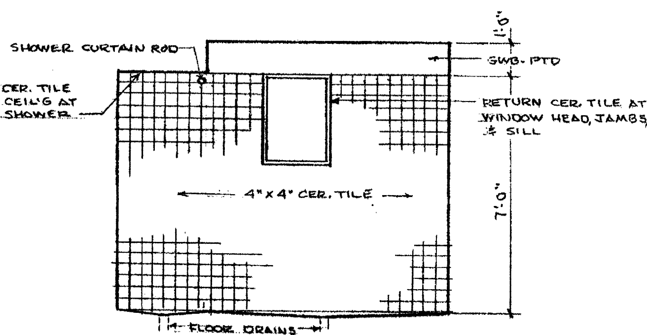
NEW BATH ELEVATIONS AT SPECIAL CARE RM
