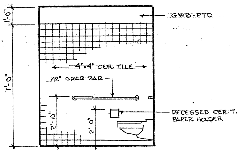
HP TOILET AT BATHING AREA
