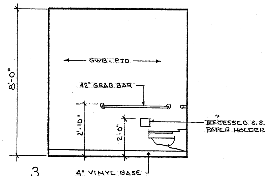
TYP. VISITOR HP TOILET AT CENTRAL CORE
