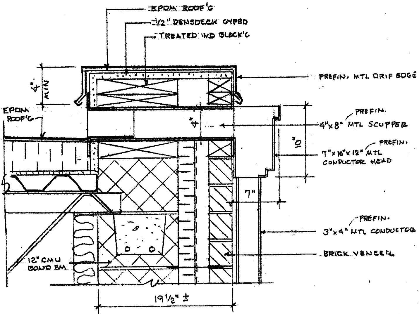
METAL ROOF SCUPPER & CONDUCTOR DETAIL
