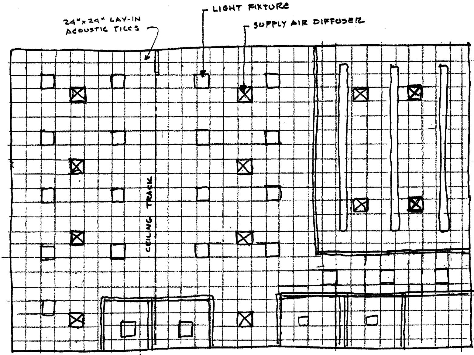
REFLECTED CEILING PLAN AT NEW ADDITION.
